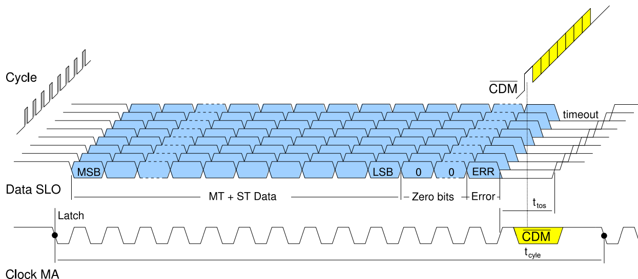
Figure 17: Example of SSI line signals (MODEA=0x5/0x6) with optional unidirectional register communication
