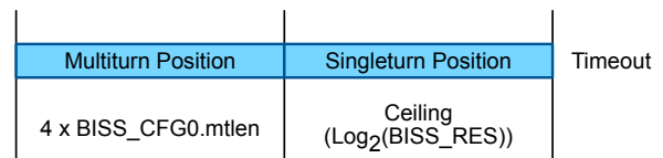
Figure 17: SSI Frame Format
