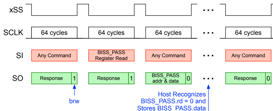
Figure 18: BiSS Passthrough Write
