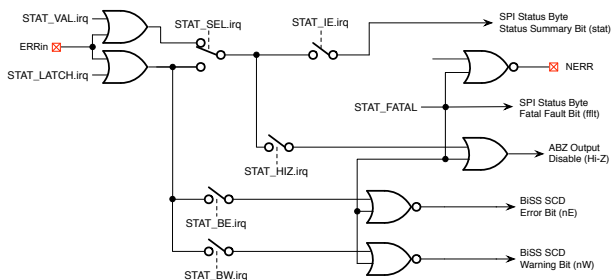
Figure 24: Interrupt Request Using NERR
