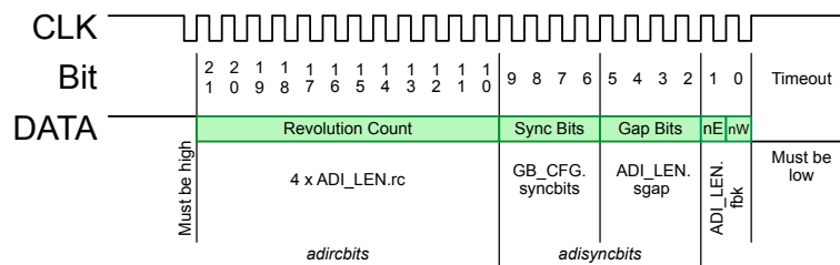
Figure 21: Expected SSI Data Frame
