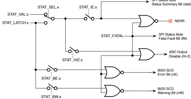
Figure 23: Single Condition Status and Fault Logic
