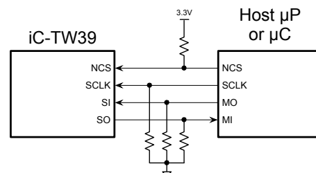
Figure 10: SPI Port Connection
