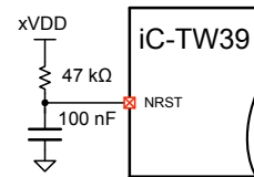
Figure 9: NRST Connection
