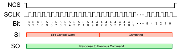
Figure 28: Command Packet Format
