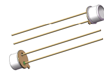
TO46-2F ∅ 4.7 mm, h 3.7 mm RoHS compliant
