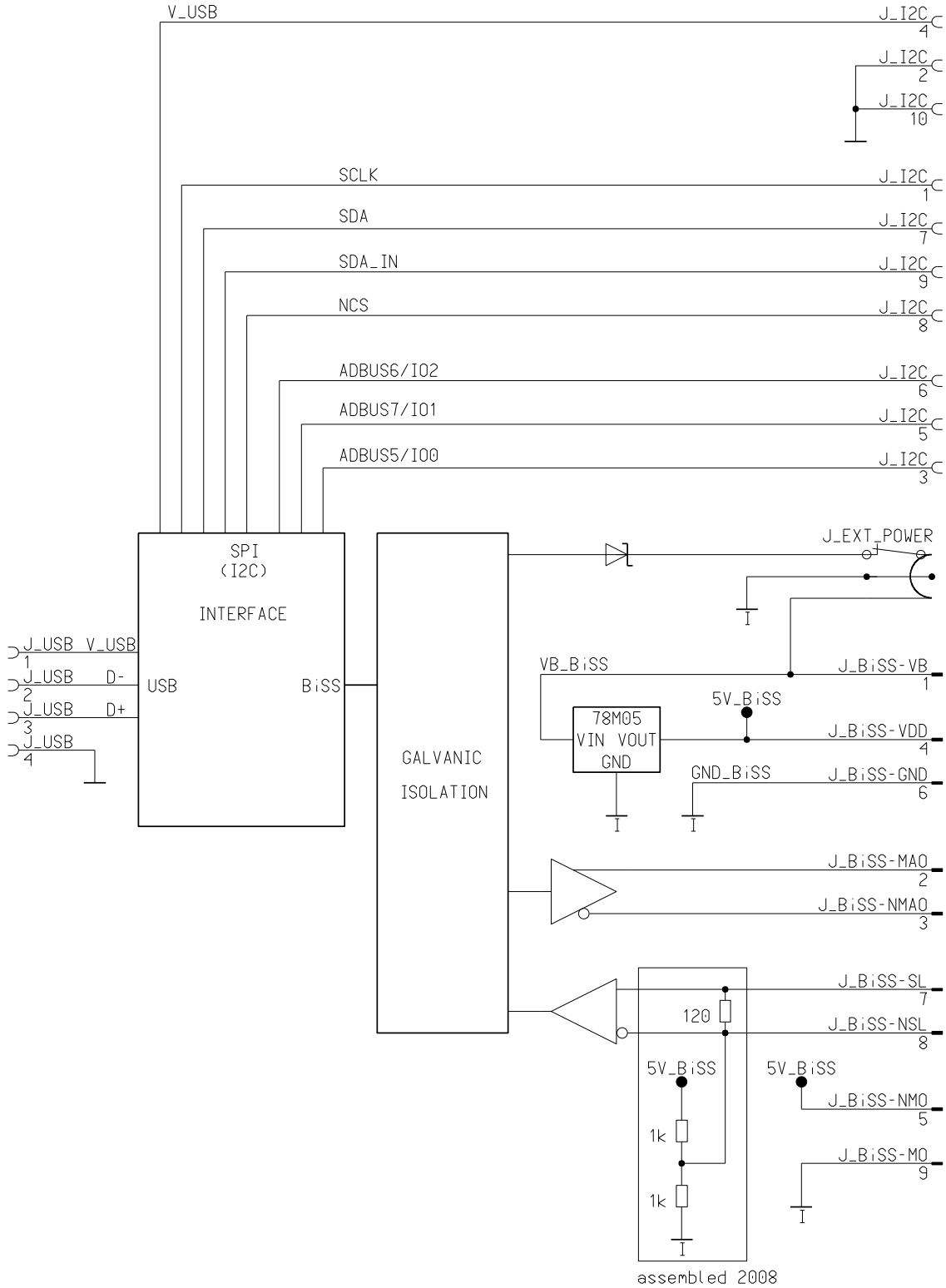
Figure 2: Power supply routing of MB3U-I2C
