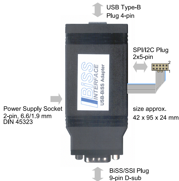
Figure 1: iC-MB3 iCSY MB3U-I2C
