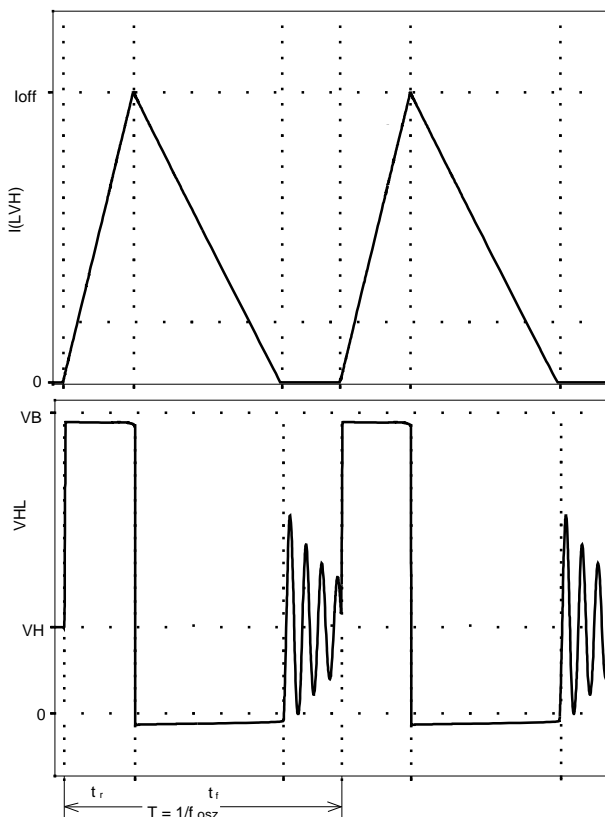
Figure 6: Intermittent flow
