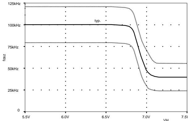
Figure 5: Oscillator Frequency
