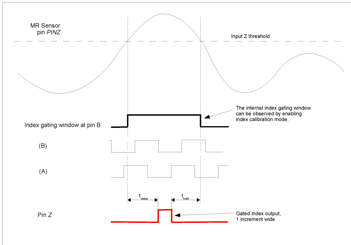
Figure 6: Example of correctly set threshold when using an MR gating sensor. The side lobes are below the threshold line and no parasitic triggering occurs.
