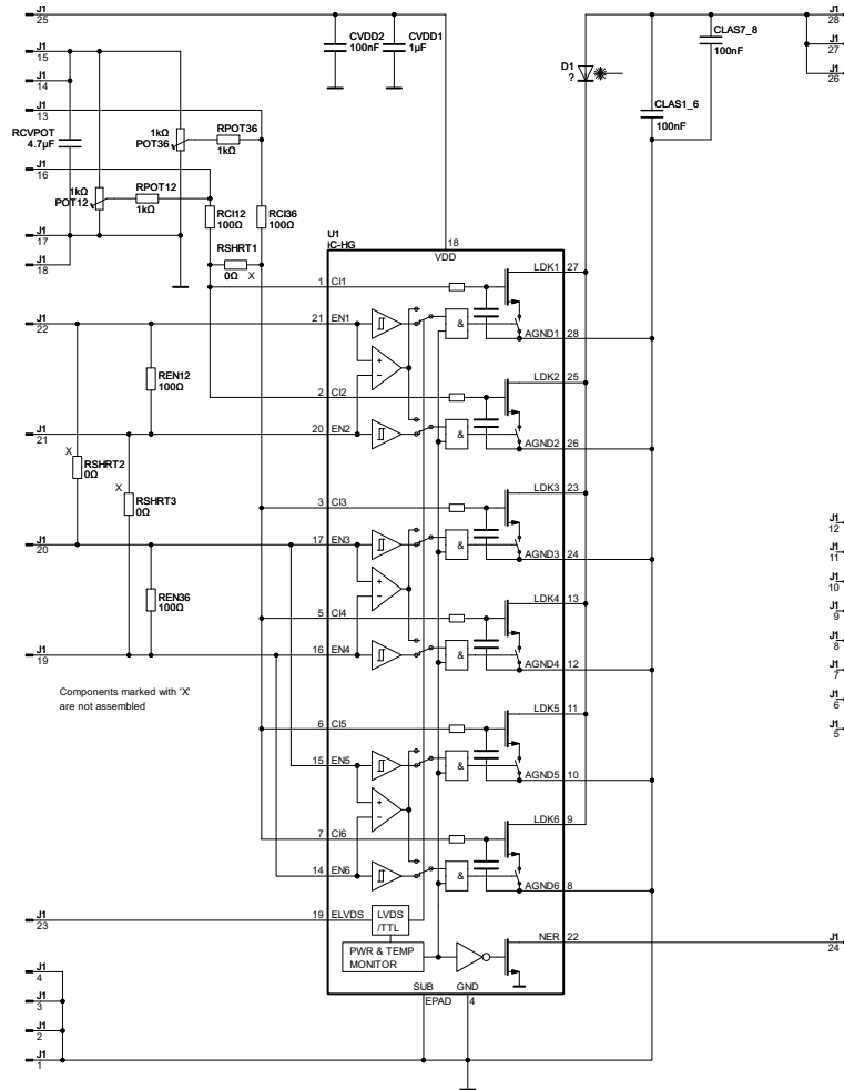
Figure 5: Circuit diagram
